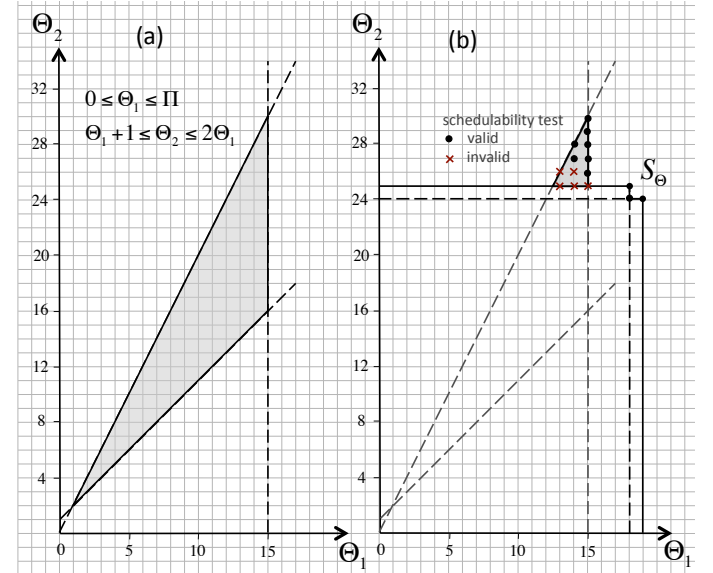
Figure 7: The example of a GMPR interface computation
