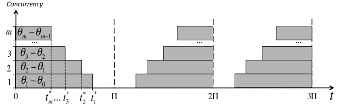
Figure 4: The worst-case supply allocation under the GMPR model
