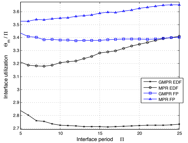
Figure 8: Case (a): m = 4 , U_{max} = 0.4 , \frac{T_{max}}{T_{min}} = 1.5 .
