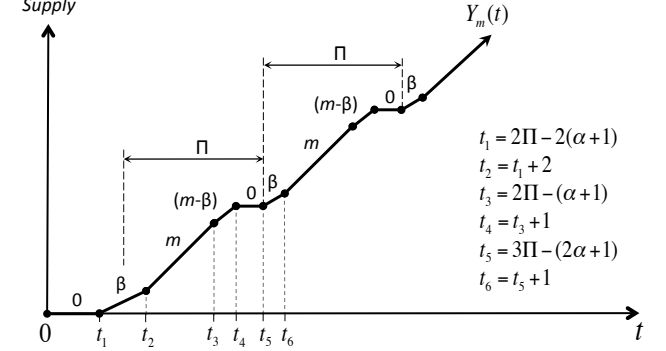
Figure 3: The worst-case supply allocation under the MPR model
