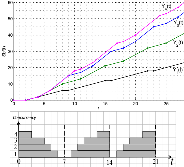
Figure 5: The PSF (top) and the worst-case supply pattern (bottom) of the GMPR interface \langle 7, \{6, 11, 15, 17\} \rangle . The bold points indicate the slope change of the PSF functions.
