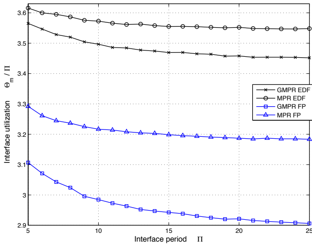
Figure 11: Case (d): m = 4 , U_{\max} = 0.4 , \frac{T_{\max}}{T_{\min}} = 100 .
