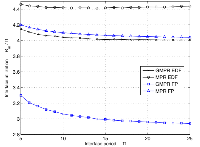
Figure 12: Case (e): m = 5 , U_{\max} = 0.4 , \frac{T_{\max}}{T_{\min}} = 100 .
