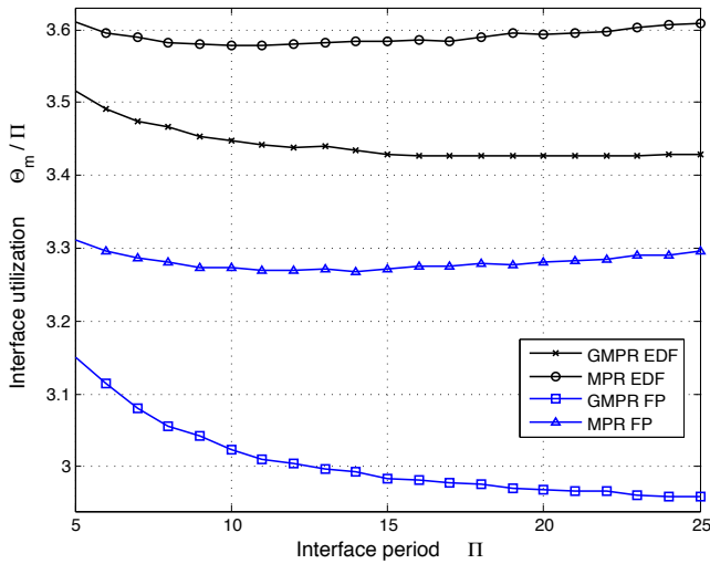
Figure 10: Case (c): m = 4 , U_{\max} = 0.4 , \frac{T_{\max}}{T_{\min}} = 10 .
