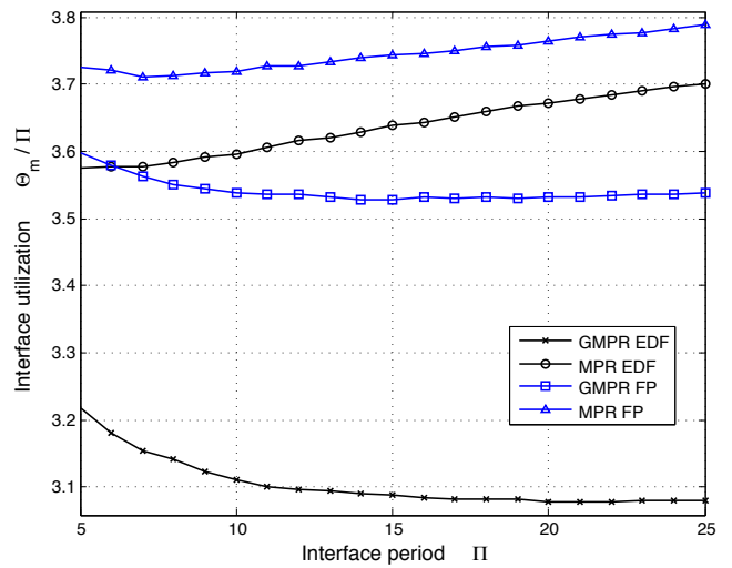
Figure 9: Case (b): m = 4 , U_{max} = 0.7 , \frac{T_{max}}{T_{min}} = 1.5 .
