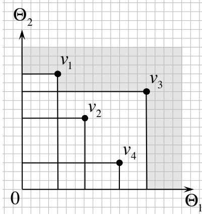
Figure 6: Illustration of the search space reduction.
