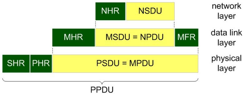
Figure 2.1: Structure of the IEEE 802.15.4/ZigBee frames.
