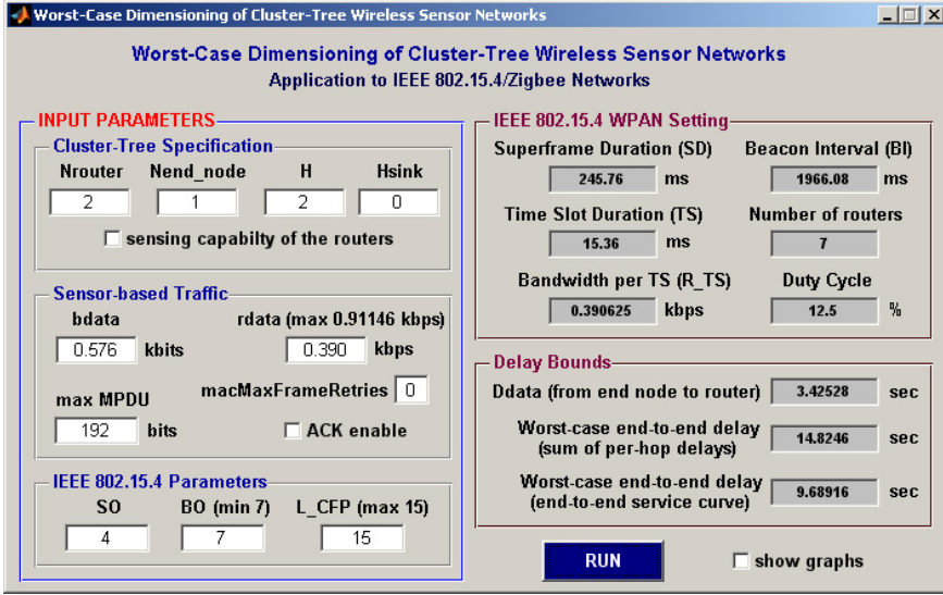
Figure 5.11: The GUI of the Matlab analytical model.
