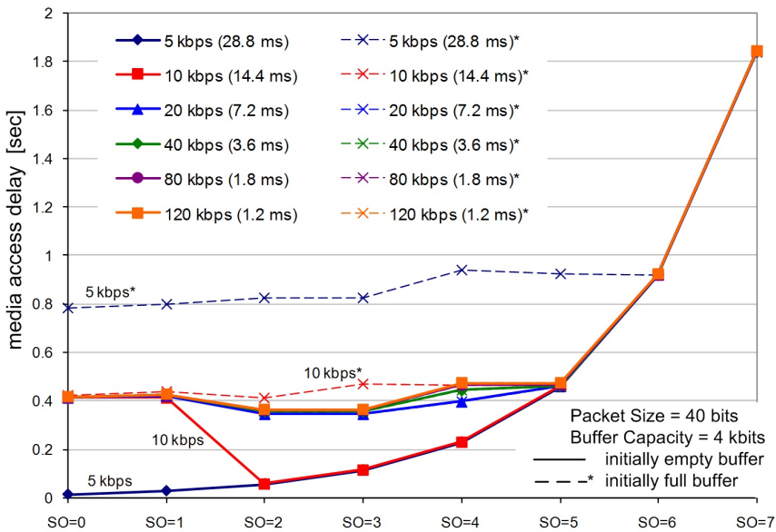
Figure 3.8: The media access delay as a function of the arrival data rate.
