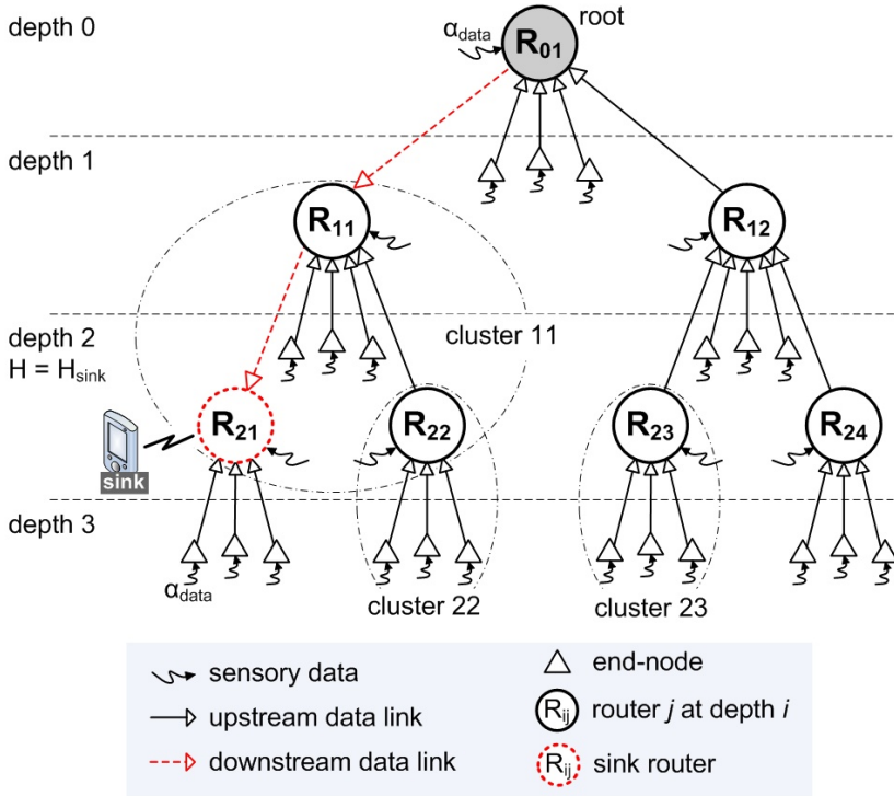
Figure 5.3: The worst-case cluster-tree topology model corresponding to a configuration where N_{\text{end-node}}^{\text{MAX}} = 3 , N_{\text{router}}^{\text{MAX}} = 2 , H_{\text{sink}} = 2 , and H = 2 .
