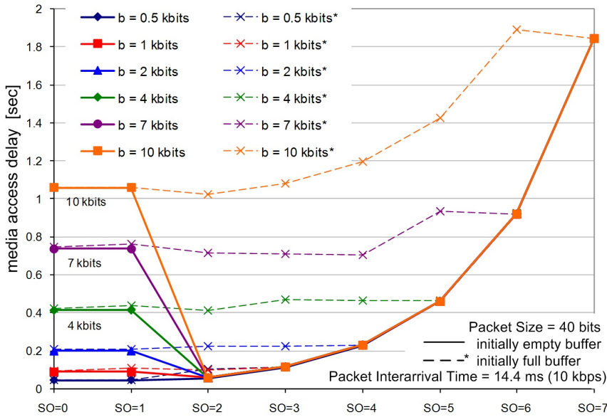
Figure 3.9: The media access delay as a function of the buffer capacity.
