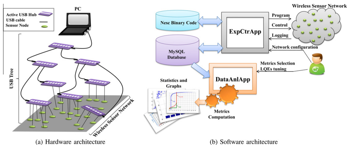
Fig. 2. RadiaLE hardware and software architectures.
