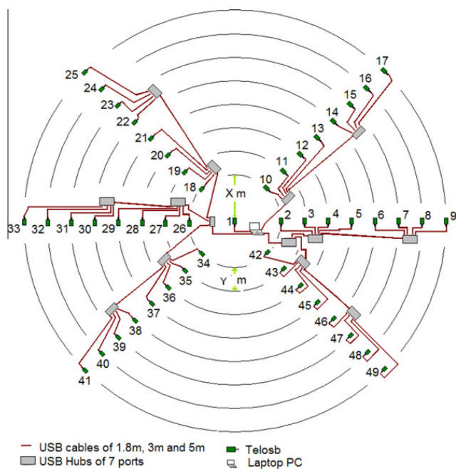
Fig. 1. Nodes distribution according to the radial topology.
