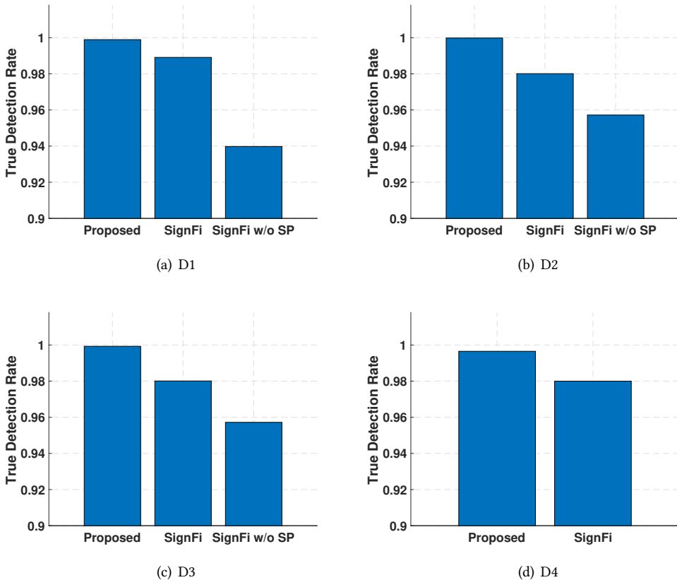
Fig. 8. The performance of true detection rate with regards to the four datasets.
