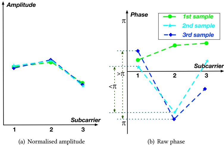
Fig. 2. Examples of data processing - Part 2
