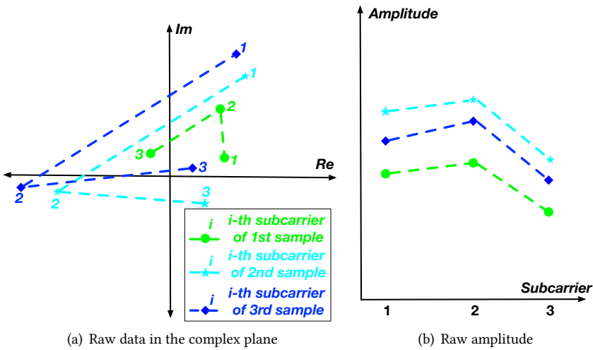
Fig. 1. Examples of data processing - Part 1
