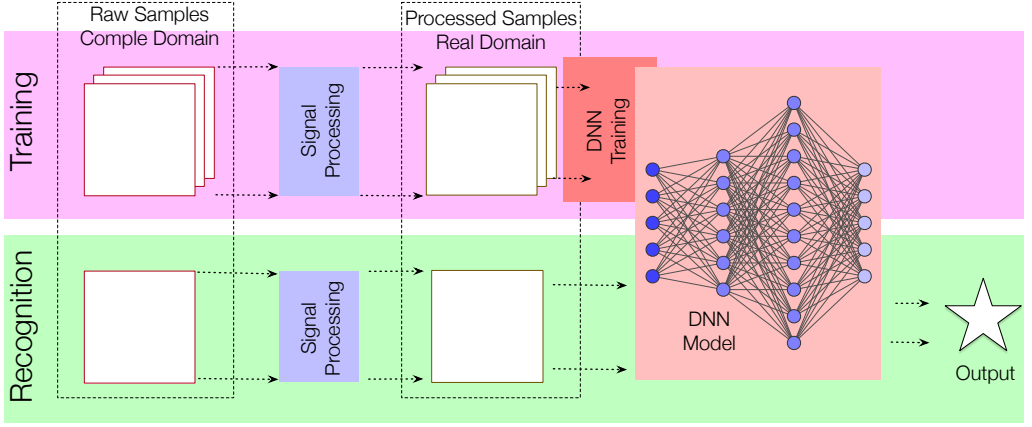
(a) Traditional DNN model
