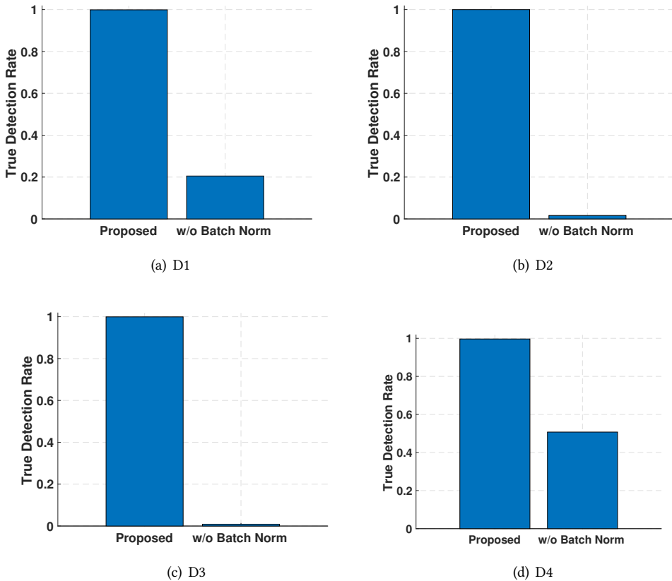
Fig. 10. The true detection rate of the proposed deep learning model with/without the batch normalisation layer.
