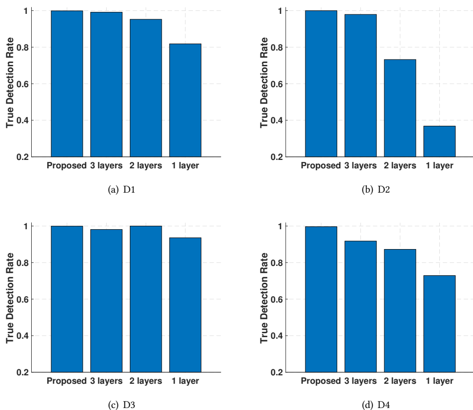
Fig. 9. The true detection rate of the proposed deep learning model with different number of Convolutional Layers
