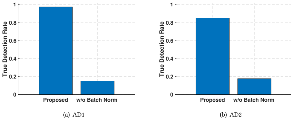
Fig. 14. The true detection rate of the proposed deep learning model with and without batch normalisation layers.
