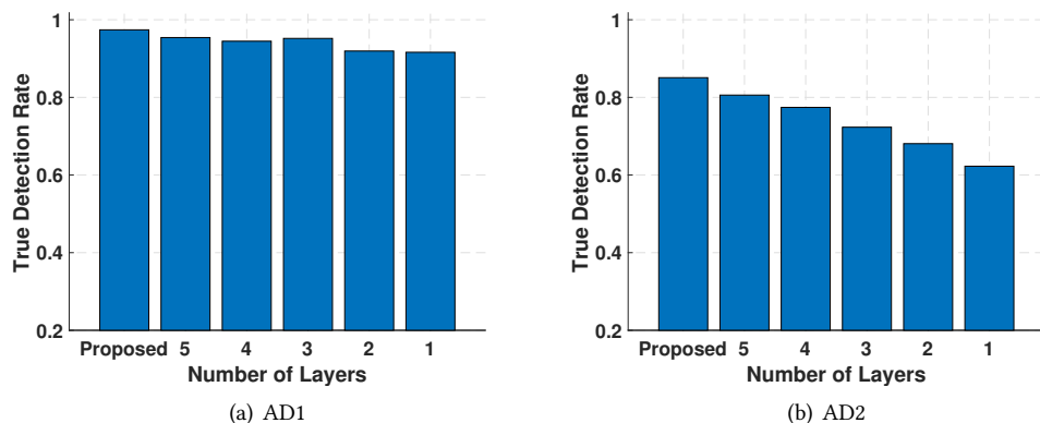
Fig. 13. The true detection rate of the proposed deep learning model with different number of Convolutional Layers
