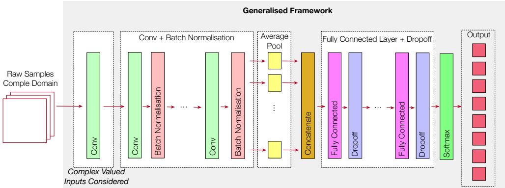
Fig. 6. The general framework for radio-based device-free context awareness
