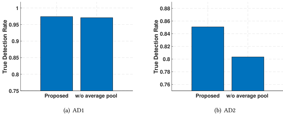
Fig. 15. The true detection rate of the proposed deep learning model with and without average pooling
