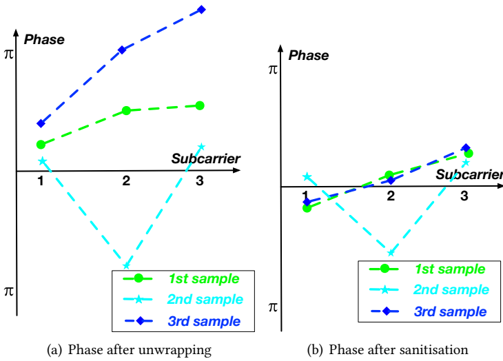
Fig. 3. Examples of data processing - Part 3
