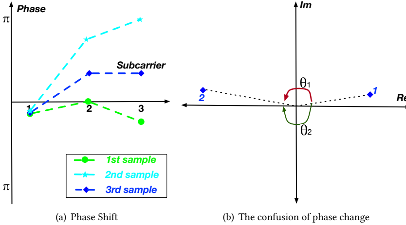
Fig. 4. Examples of data processing - Part 4
