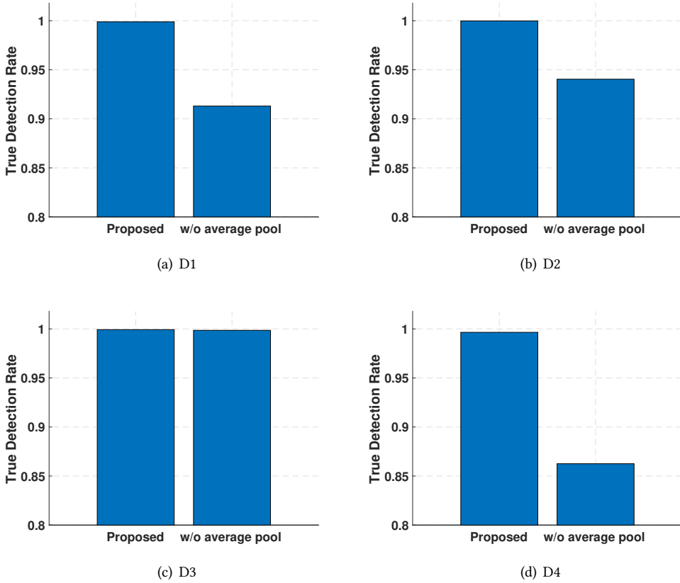
Fig. 11. The effect of average pooling
