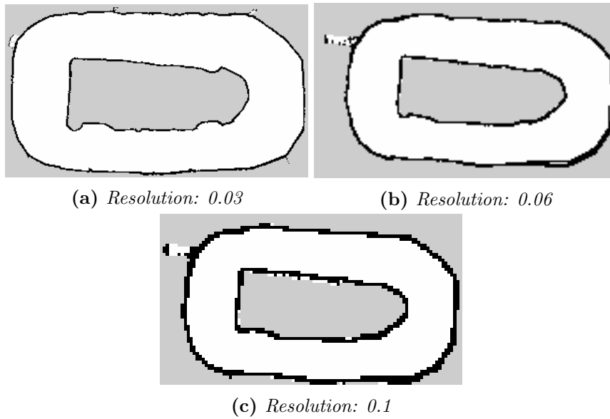
Figure 6.2: Different map generations with Hector Slam while varying their resolution.
