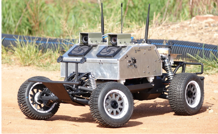
Figure 2.5: Aut rally robotic platform [5].
