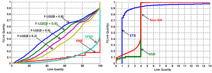
Fig. 6. Empirical CDFs of LQEs (Default Setting).
