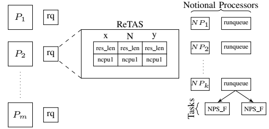
Figure 2. ReTAS Runqueue
