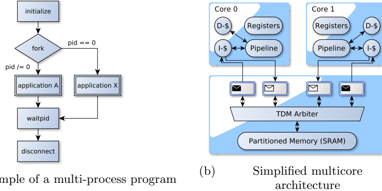
Fig. 4: Simple program running on a simplified multicore architecture
